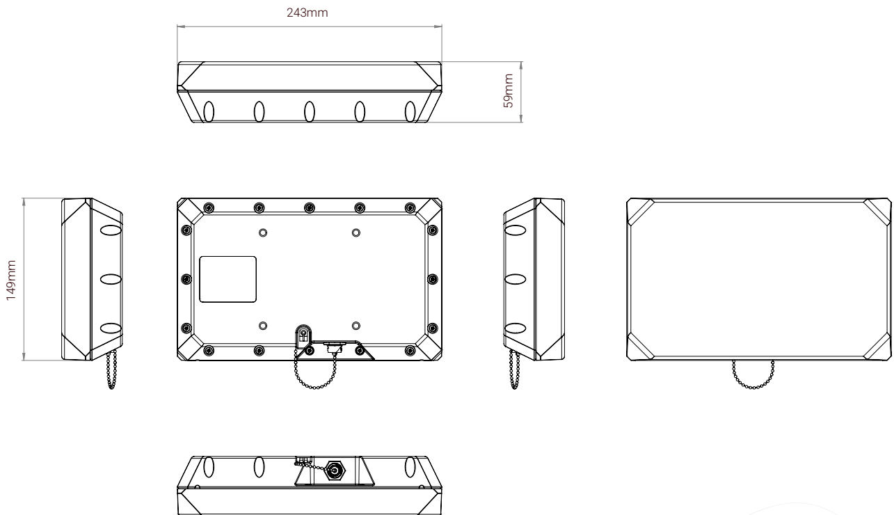
Figure 1: SR 150, 250 & 500 radar sensor outline drawing
